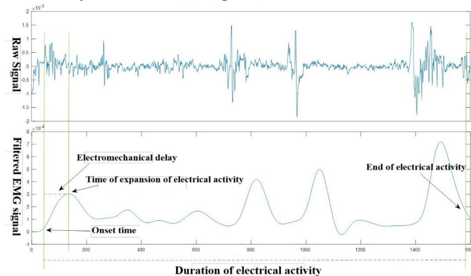
Figure 1- Onset time, Duration of electrical activity and Electromechanical delay
